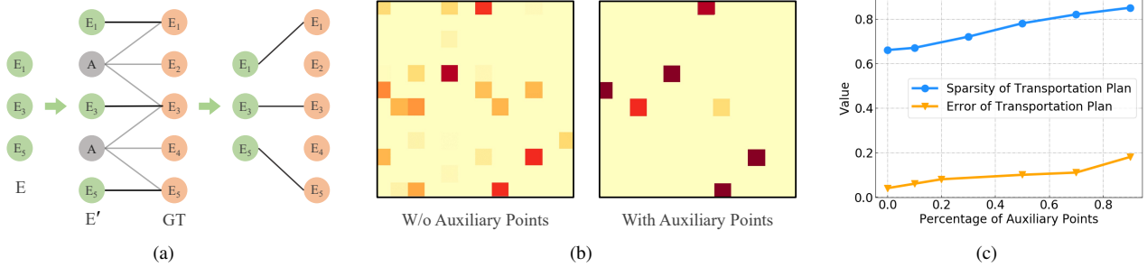
Figure 4. (a) The process to achieve sparse transportation plan through auxiliary points. E and GT are the estimated needlet coefficients and the ground truth, respectively. ‘A’ denotes the auxiliary point. E’ denotes the predicted coefficients extended with auxiliary points. The connection between E’ and GT signifies the resulting transportation plan. (b) Transportation plans for the needlet coefficients ( j=1 ) w/o and w/ auxiliary points, respectively. (c) The sparsity and error of transportation plan matrix with different percentage of auxiliary points.
